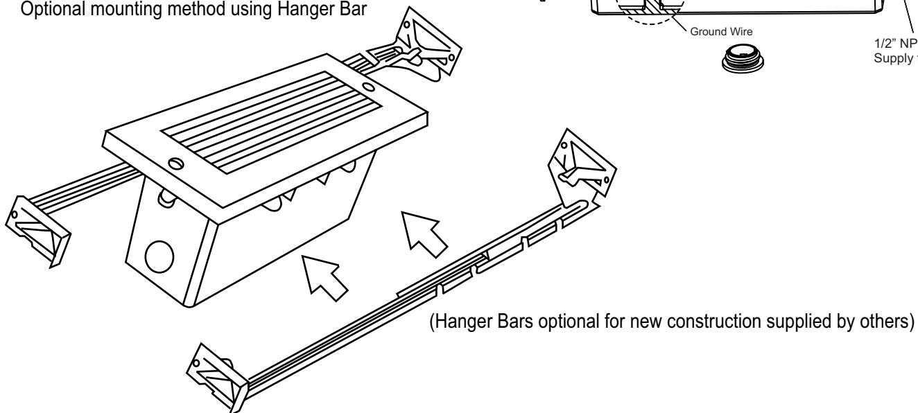
Optional mounting method using Hanger Bar
